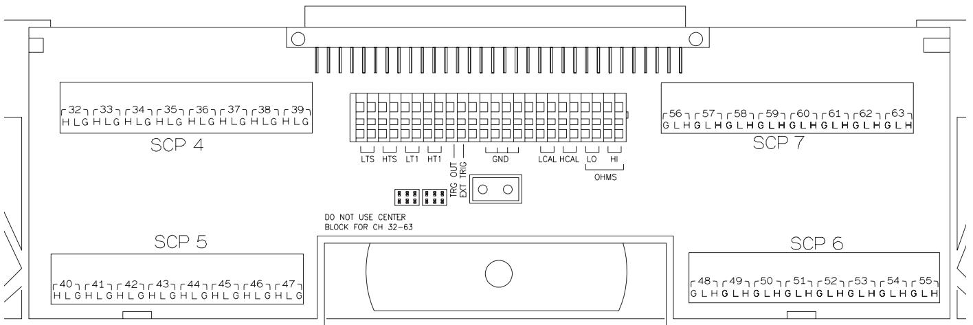
Figure 3: VT1501A B-size Terminal Module Connections (Ch 32-63)
